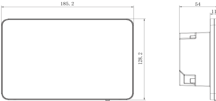
Fig.1.2 Dimension of Centralized Controller
